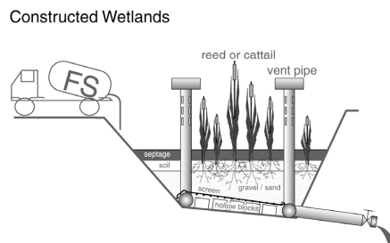
Figure 5 Pilot-scale constructed wetlands treating septage at the Asian Institute of Technology (Bangkok/Thailand)
